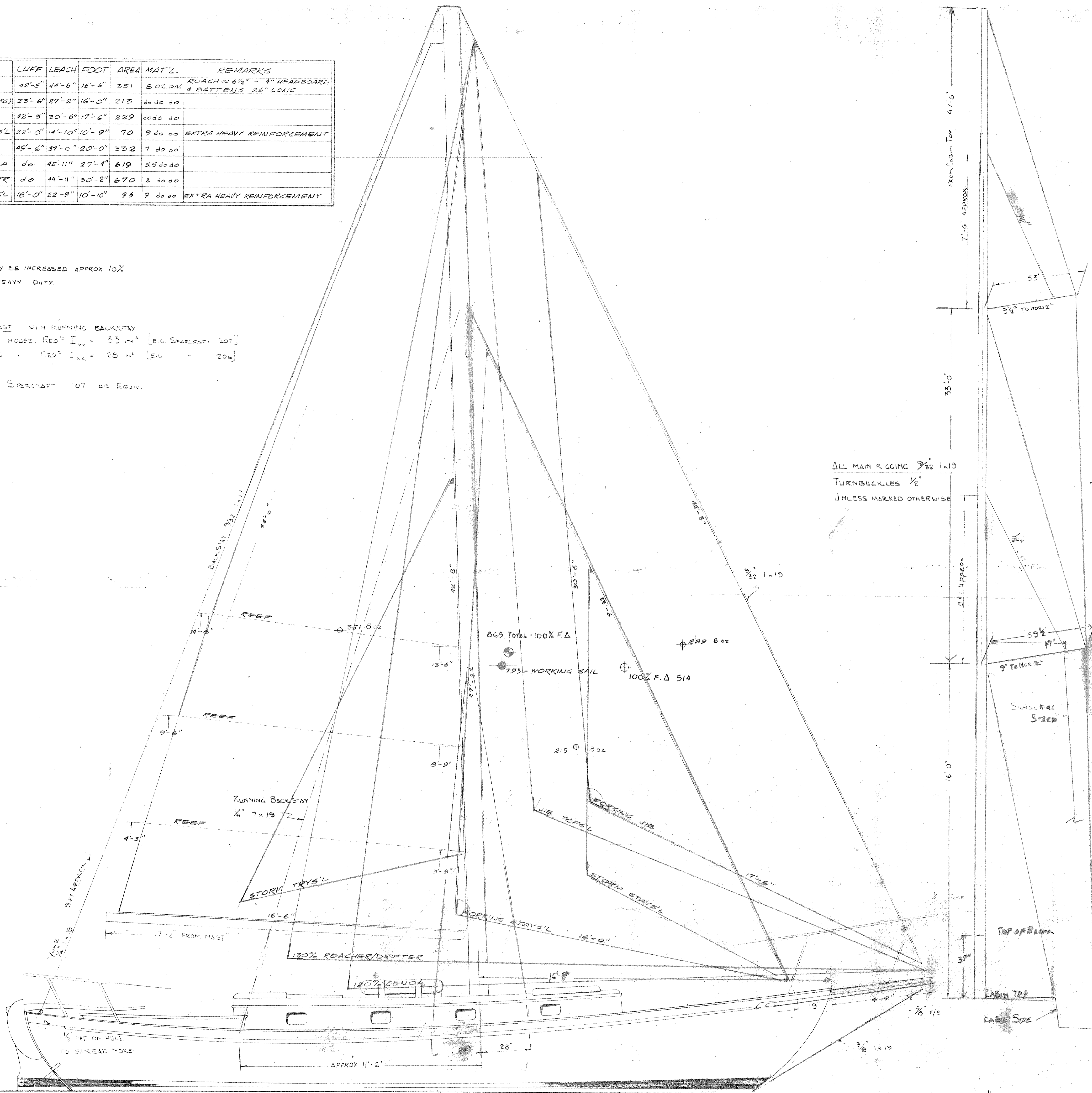
SAIL PLAN FOR AN "INGRID" TYPE CUTTER
